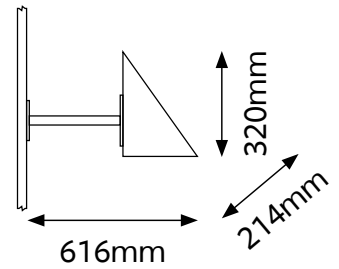
300mm Outreach Arm. To be ordered separately, Code: FIX-0476.
