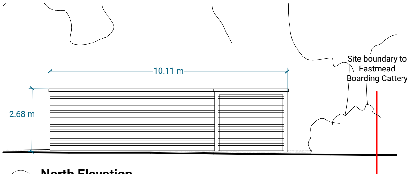
1 North Elevation 1 : 100
