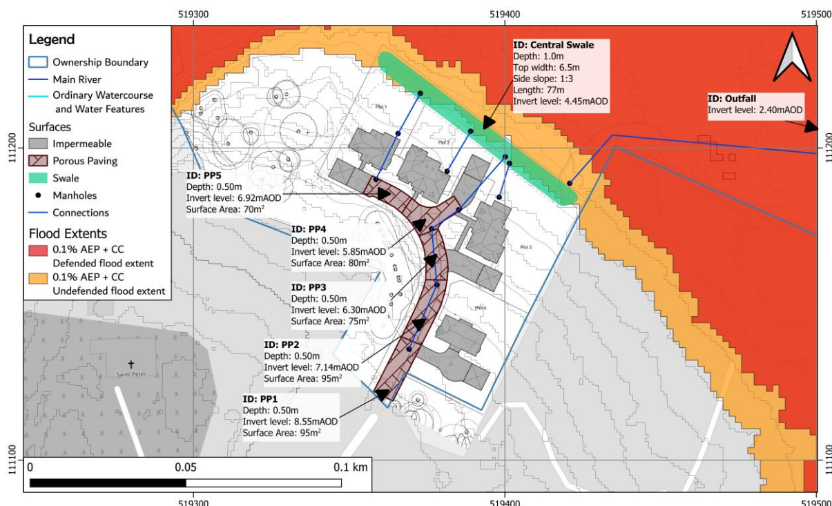
Figure 6-2 Properties of key SuDS features
