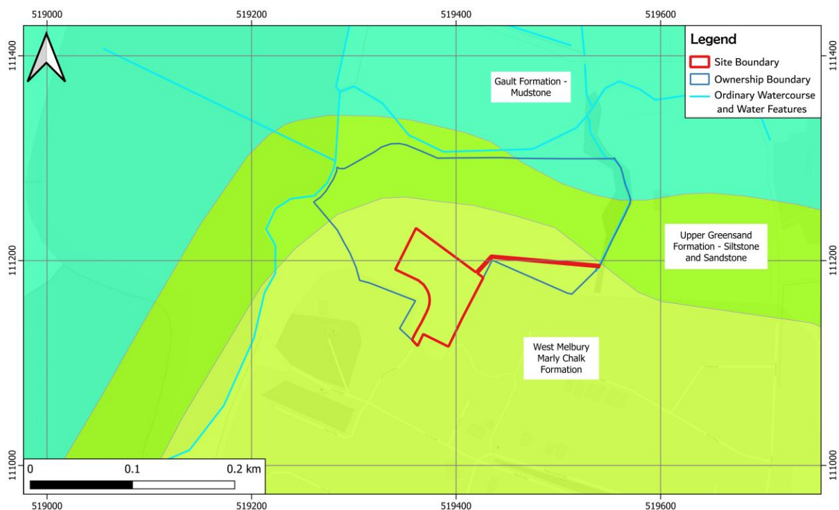
Figure 2-4 Bedrock Geology
