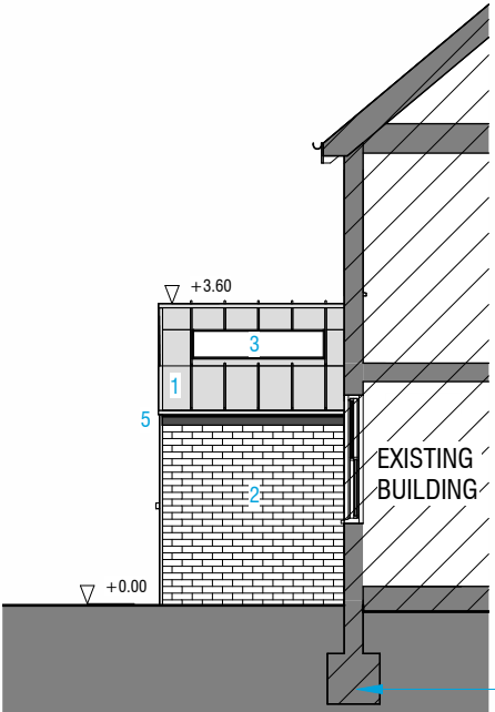
4 SHORT SIDE ELEVATION 1 : 100
