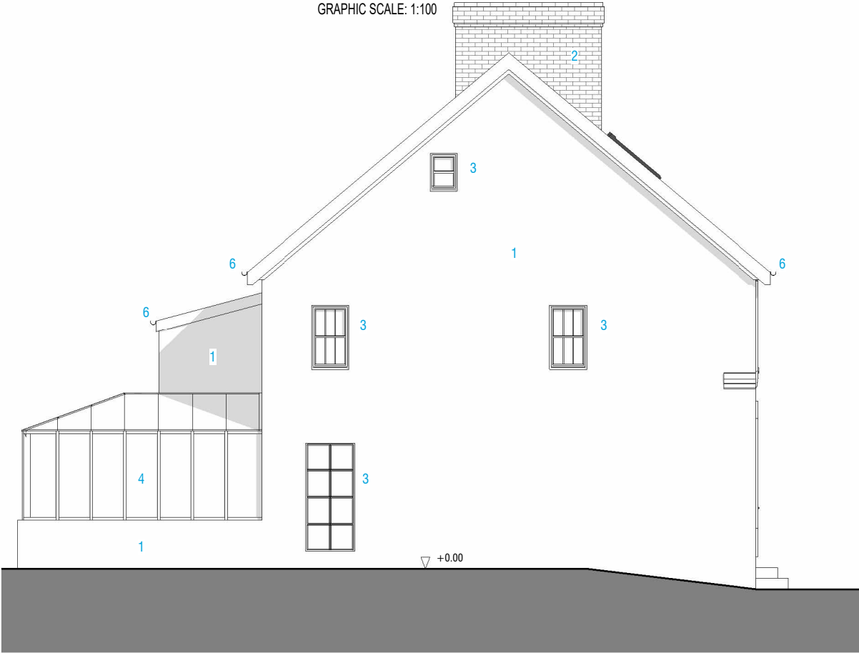
4 SIDE ELEVATION - WEST 1 : 100
