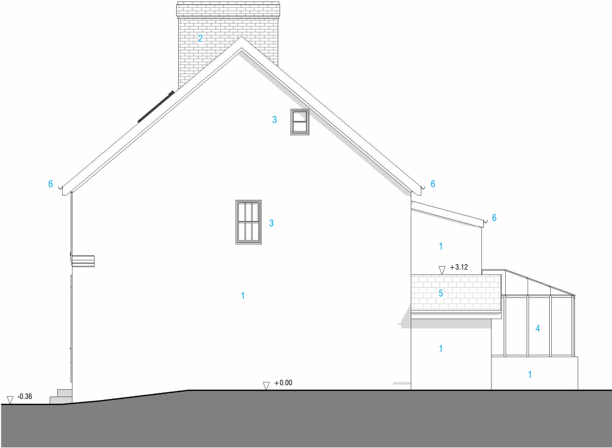
1 SIDE ELEVATION - EAST 1 : 100
