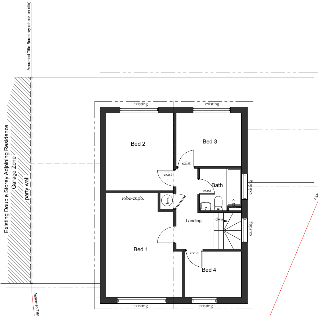
EXISTING PLAN- FIRST FLOOR SCALE 1 : 100 @ A3
