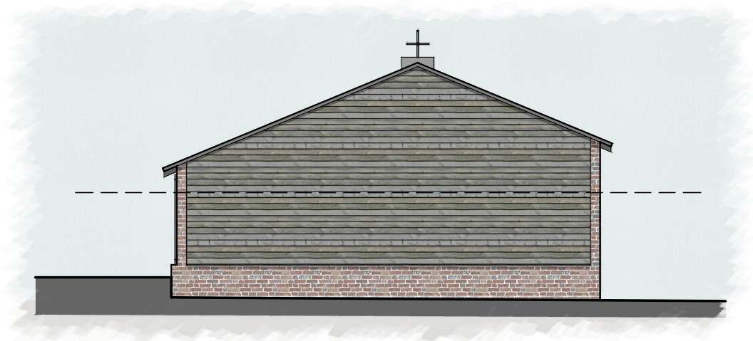
SOUTH ELEVATION
