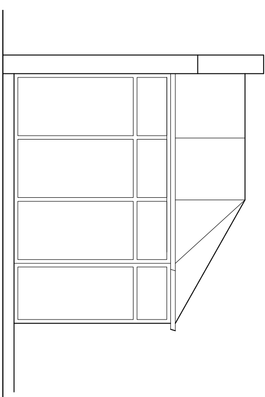
NORTH WEST: EXISTING 1:50
