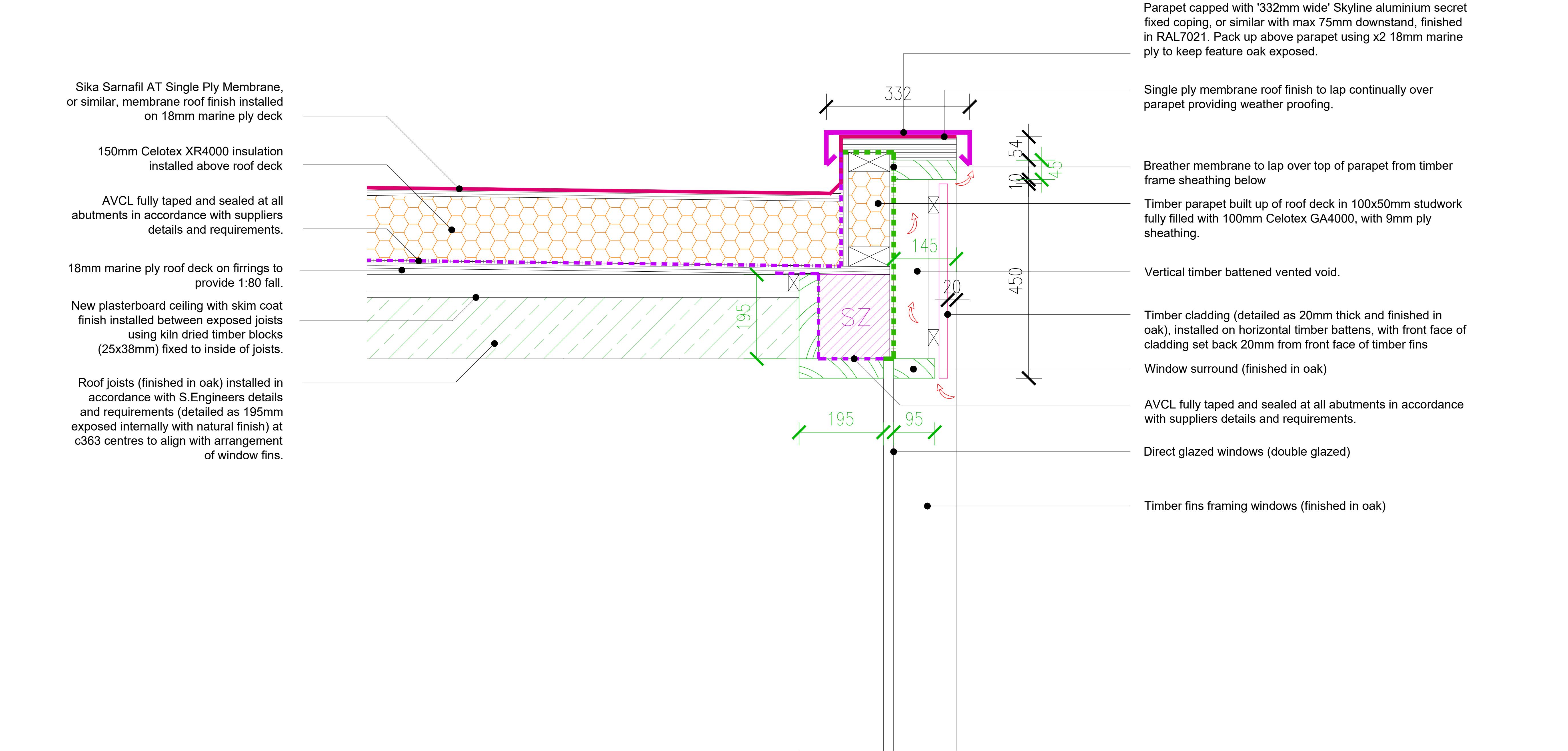
TYPICAL SECTION: EXTENSION ROOF/PARAPET 1:5
