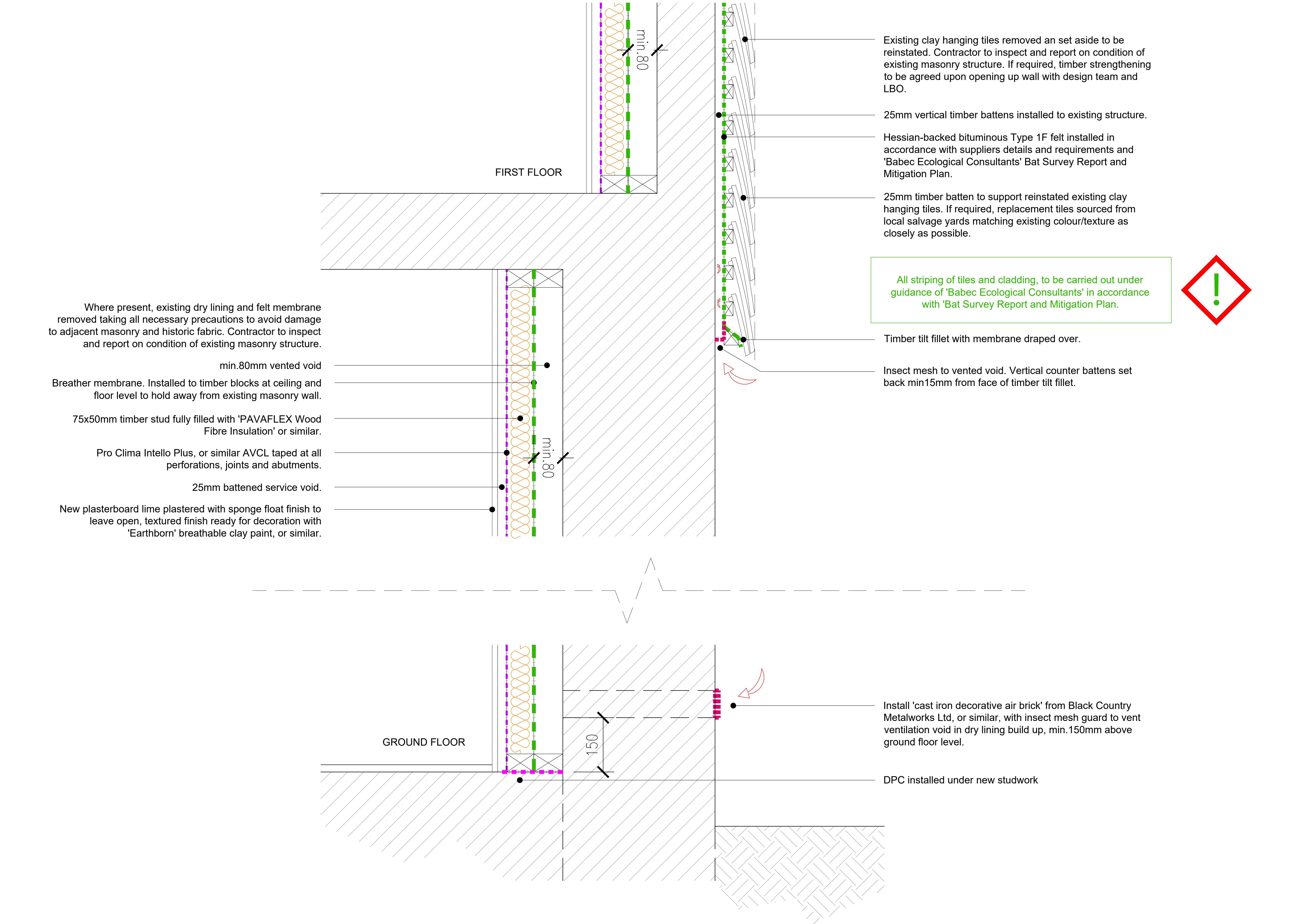
TYPICAL SECTION: INTERNAL DRY LINING AND EXTERNAL CLAY HANG TILES 1:5
