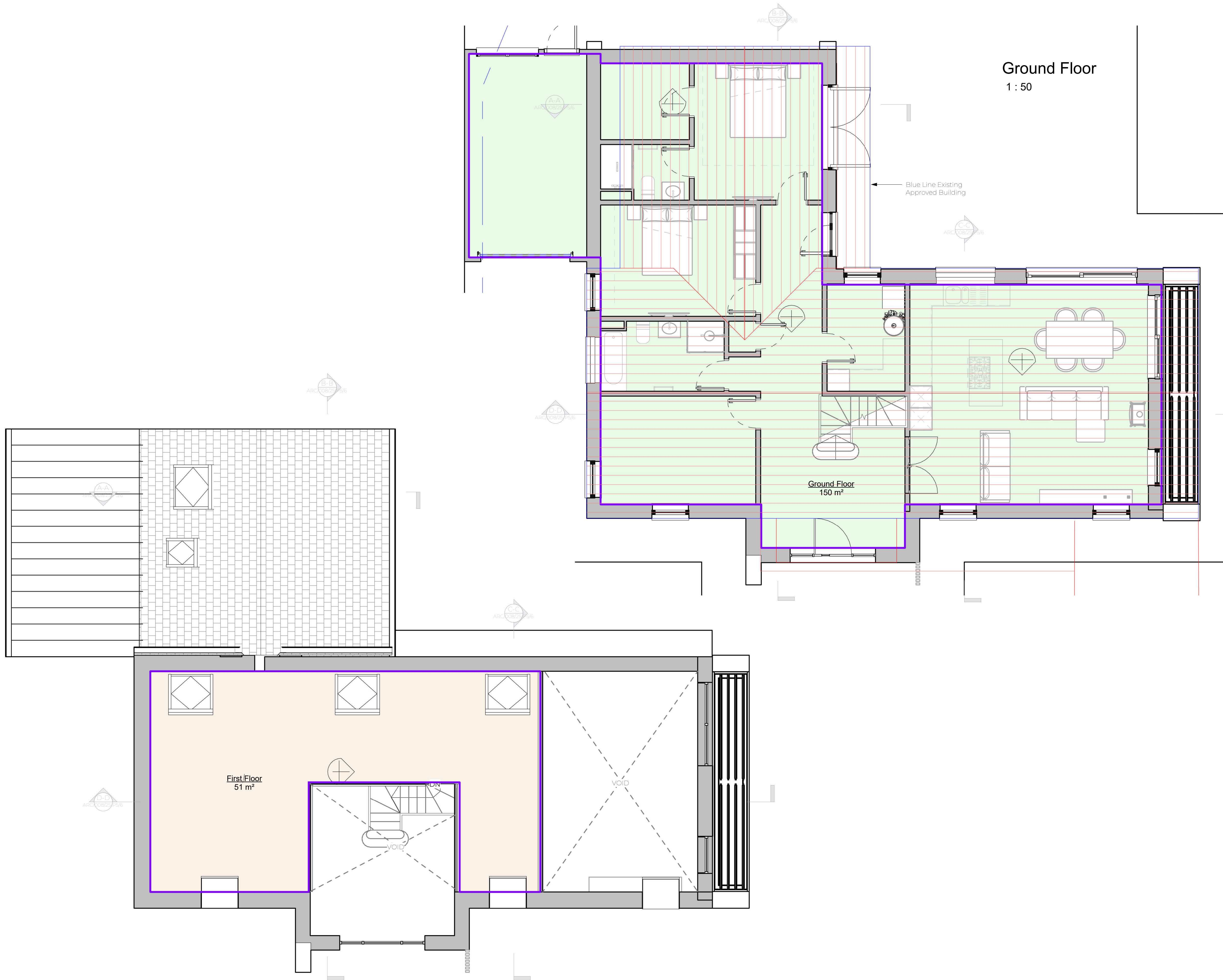
First Floor 1 : 50
