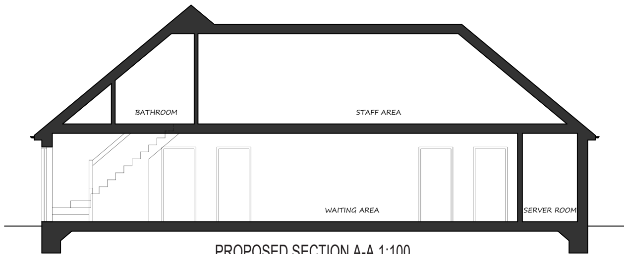
PROPOSED SECTION A-A 1:100
