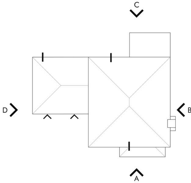
ROOF PLAN 1:200
