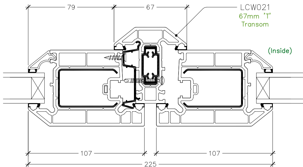
DETAIL 8
