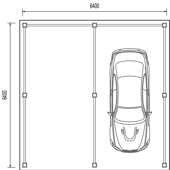
Ground Floor Plan Plots 16 -17
