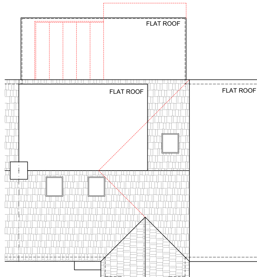
PROPOSED ROOF FLOOR PLAN
