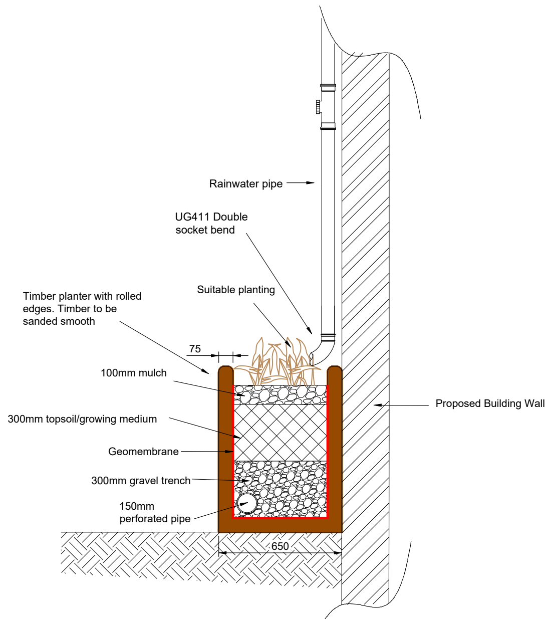
Bio-Retention Planter
