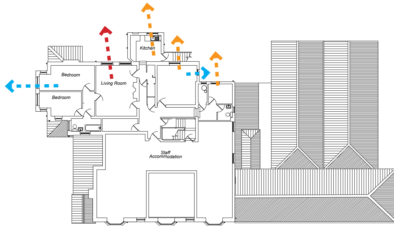
Existing First Floor
