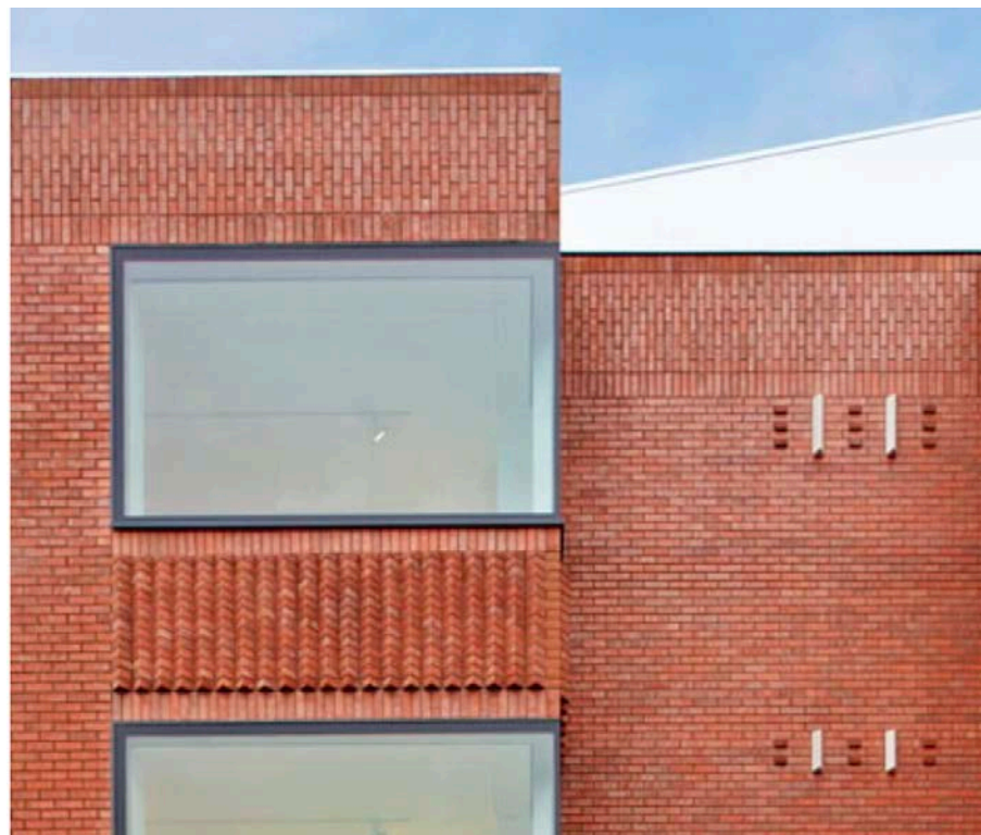
Existing soldier course detailing at the Whitworth Museum Extension in Manchester
