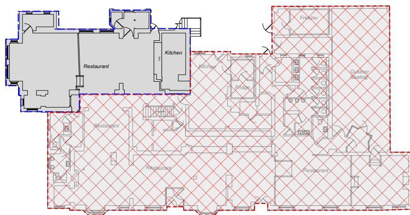
1 Ground Floor Plan Scale: 1:200
