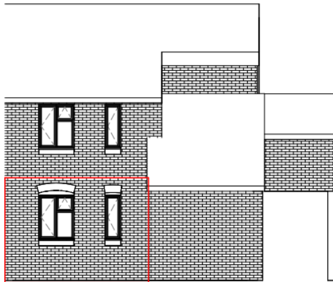
Front Existing
