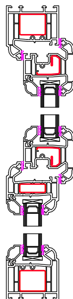
Type G - 50 - 50 Mock Sash
