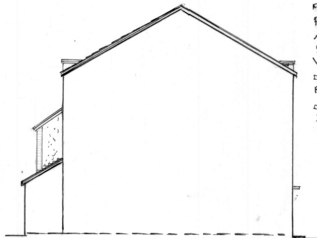
PROP. EAST ELEVATION. 1:100
