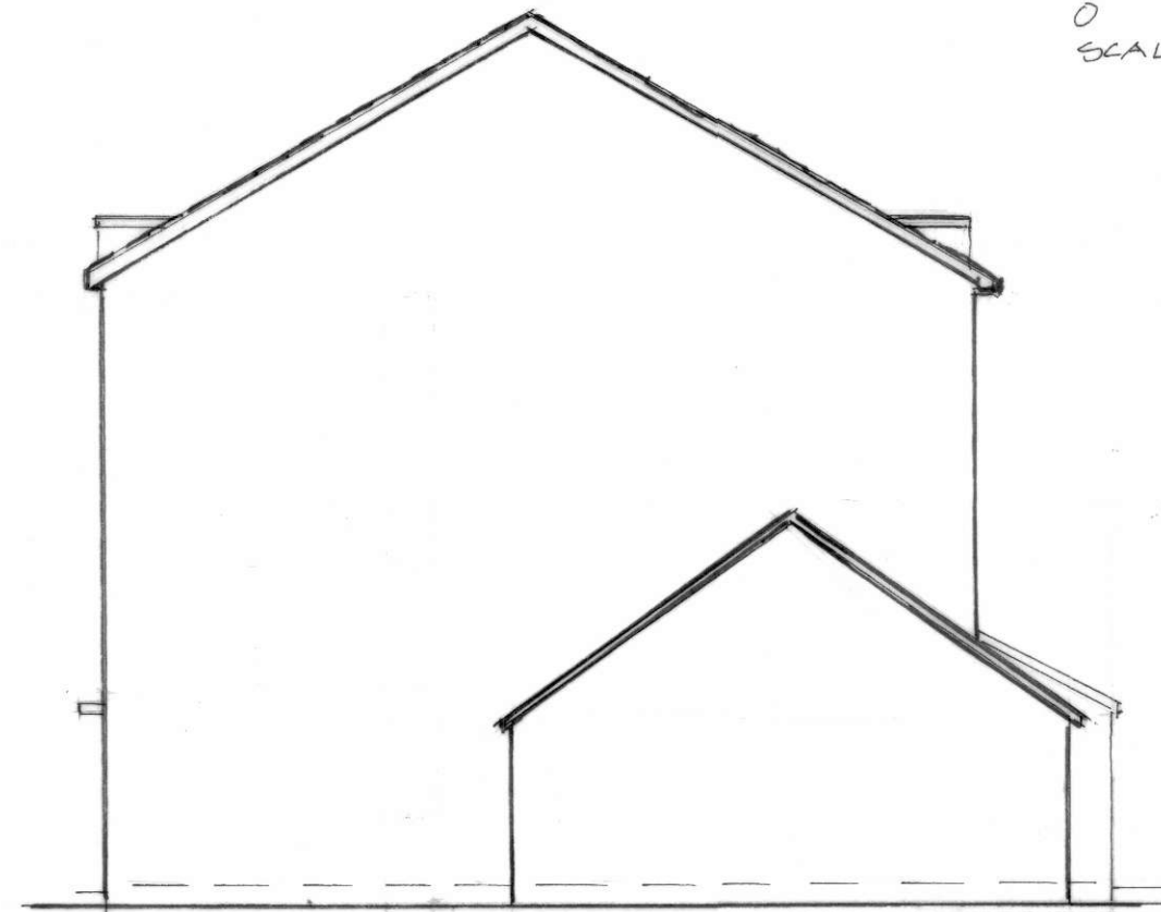
EXTG. WEST ELEVATION 1:100
