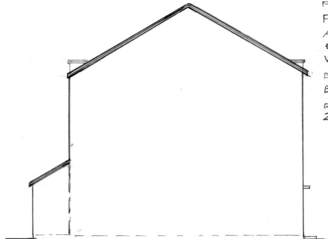
EXTG. EAST ELEVATION 1:100
