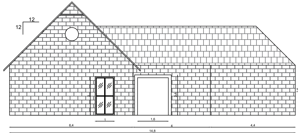
ELEVATION Scale 1: 100
