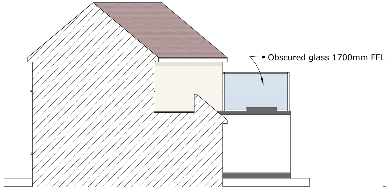
A :: Proposed South East Elevation 04 scale: 1:100
