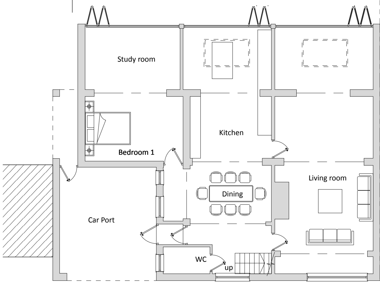
A :: Proposed Ground Floor Plan 02 scale: 1:100
