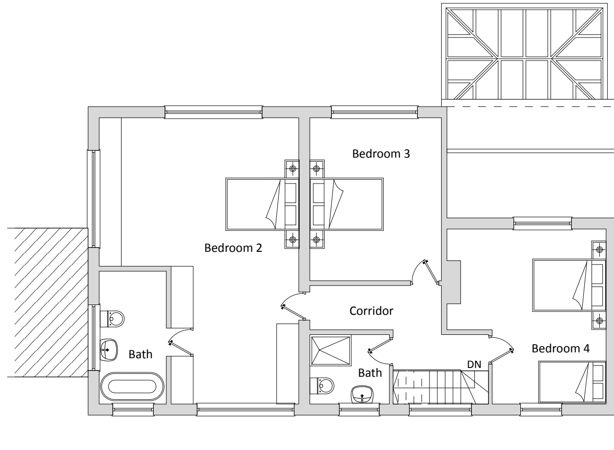
A :: Existing First Floor Plan 01 scale: 1:100
