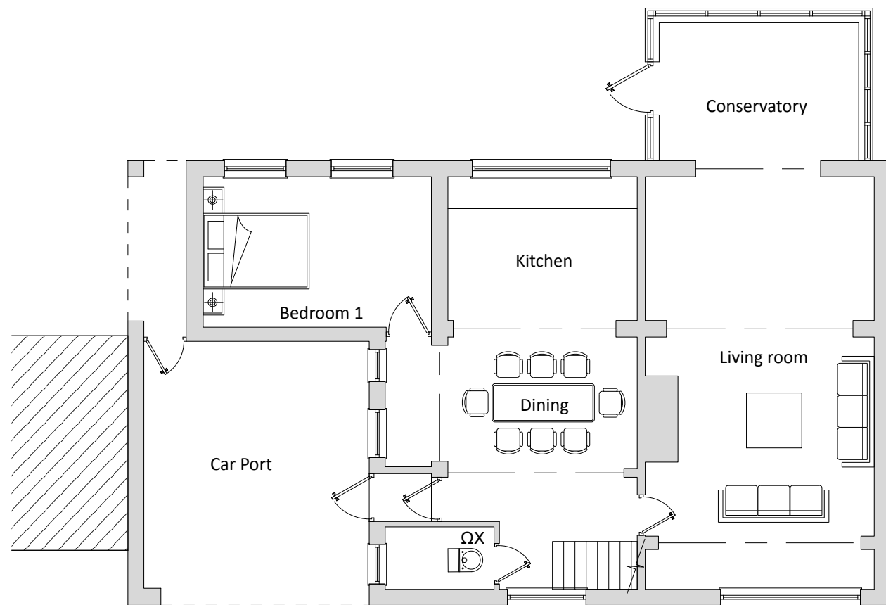
A :: Existing Ground Floor Plan 01 scale: 1:100
