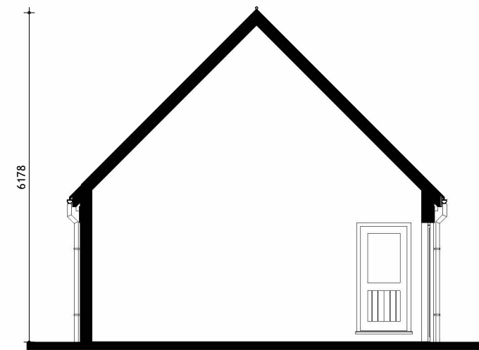
Building Section
