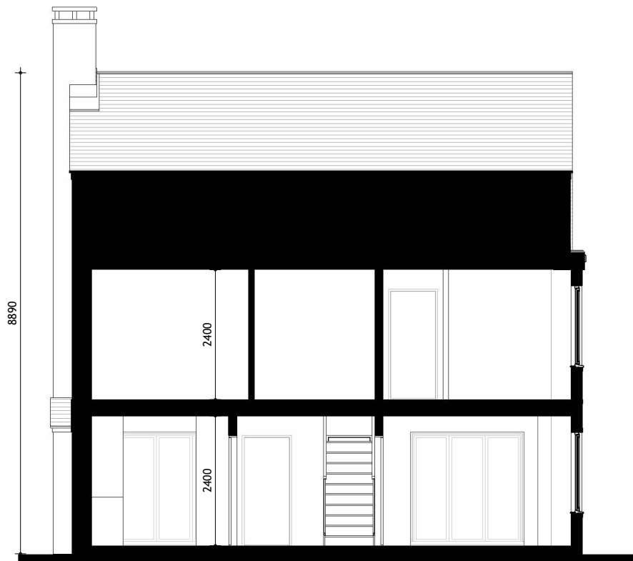
Building Section
