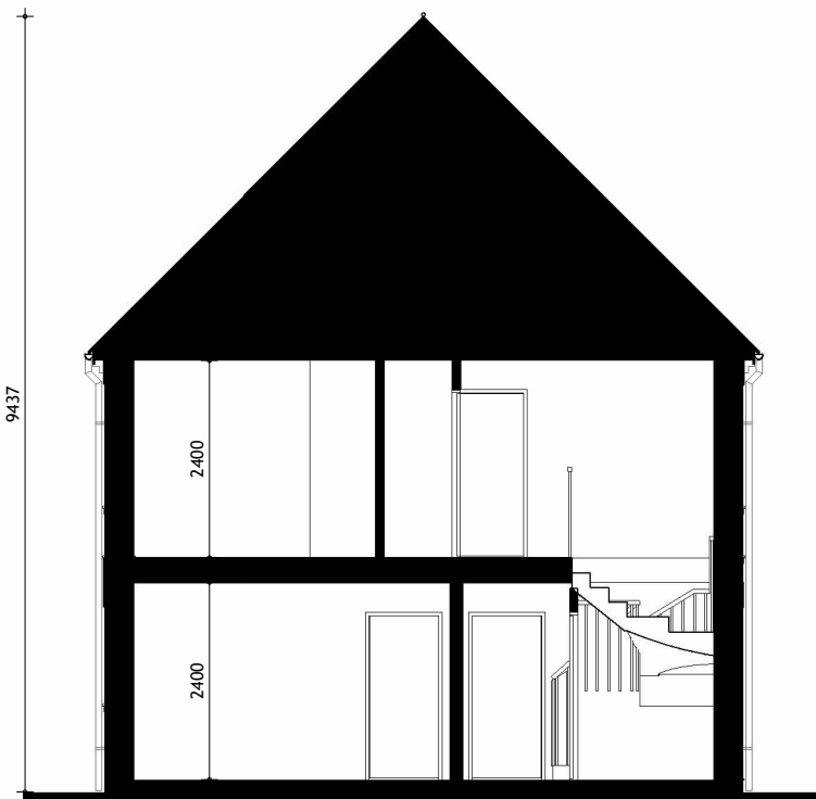
Building Section
