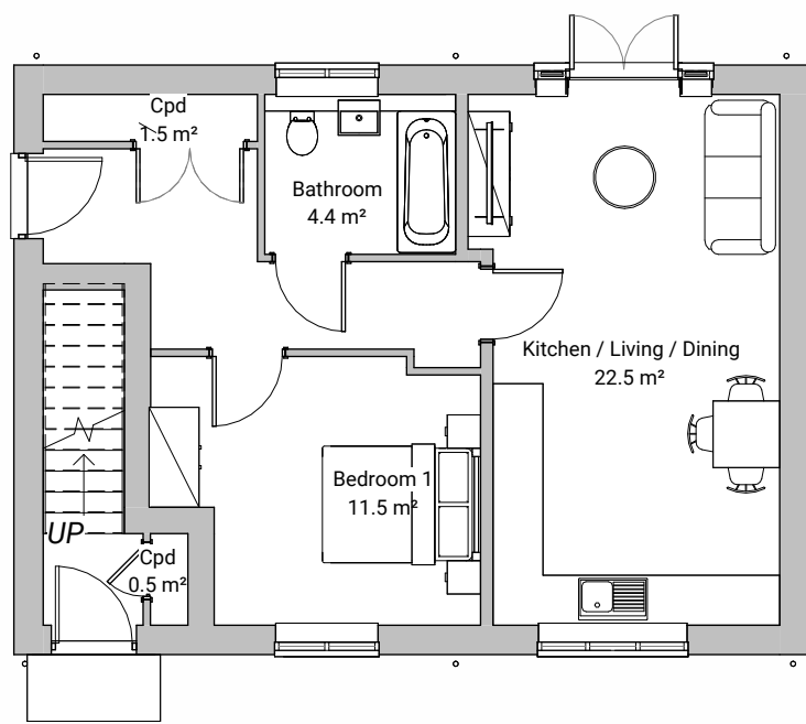
Ground Floor Plan 1 : 100
