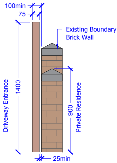
SIDE ELEVATION PROPOSED 1:25
