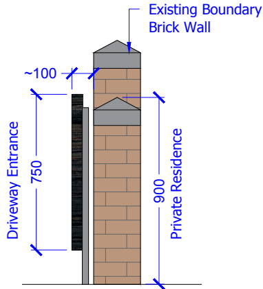
SIDE ELEVATION EXISTING
