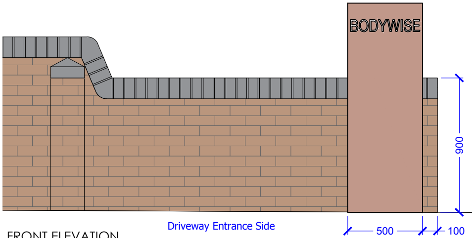
FRONT ELEVATION PROPOSED 1:25
