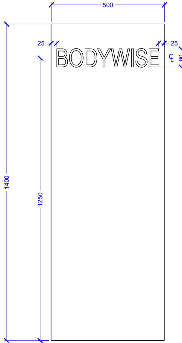
FRONT ELEVATION PROPOSED 1:10
