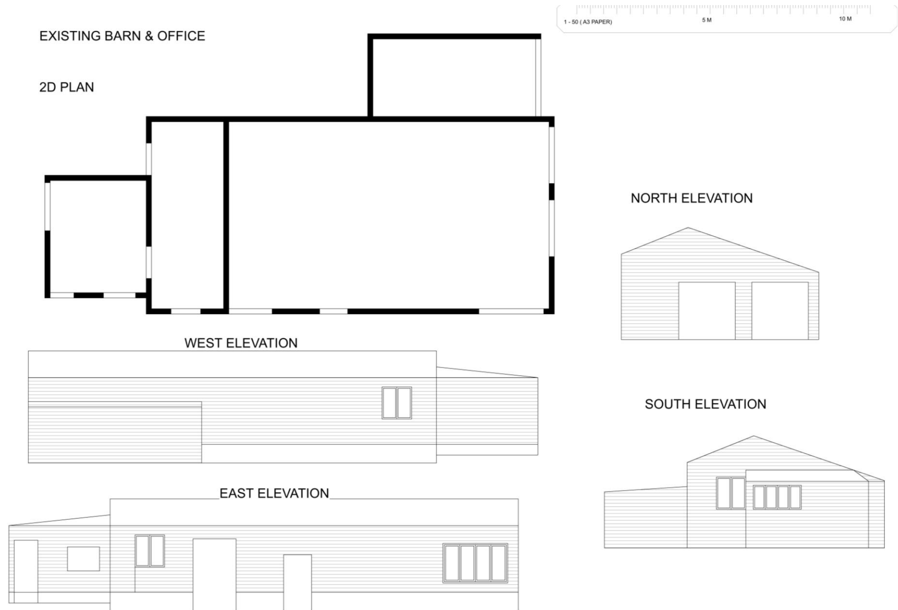
Figure 3 – Existing B1 elevations
