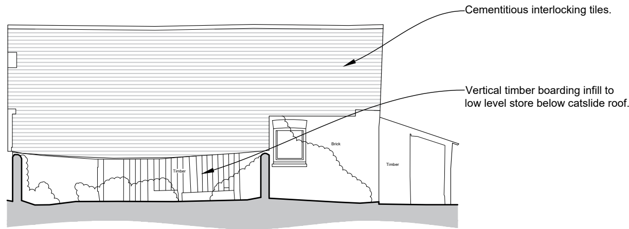
4 West Elevation 1:100 Existing
