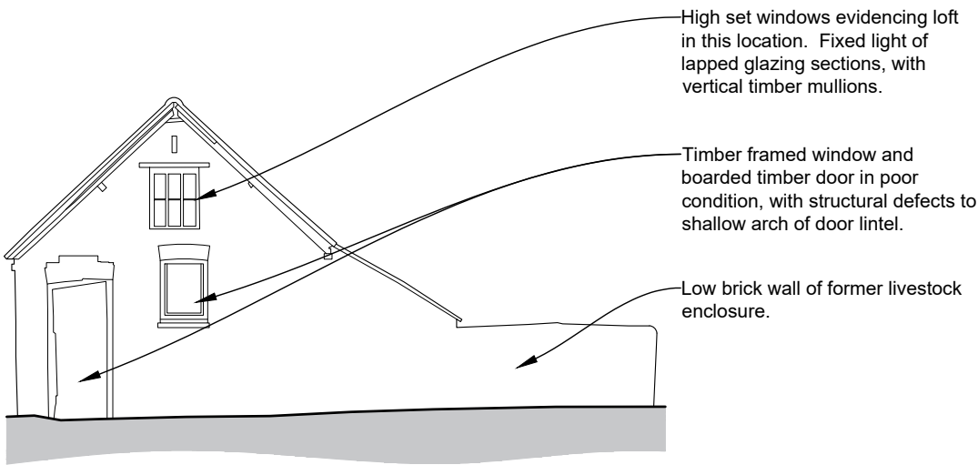
1 North Elevation 1:100 Existing
