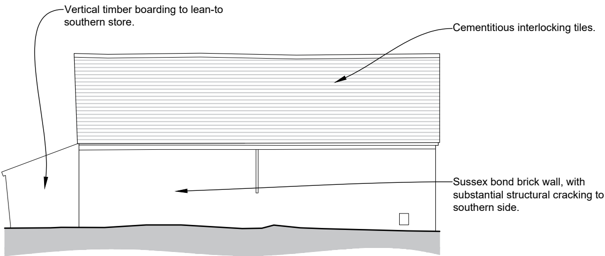
2 East Elevation 1:100 Existing
