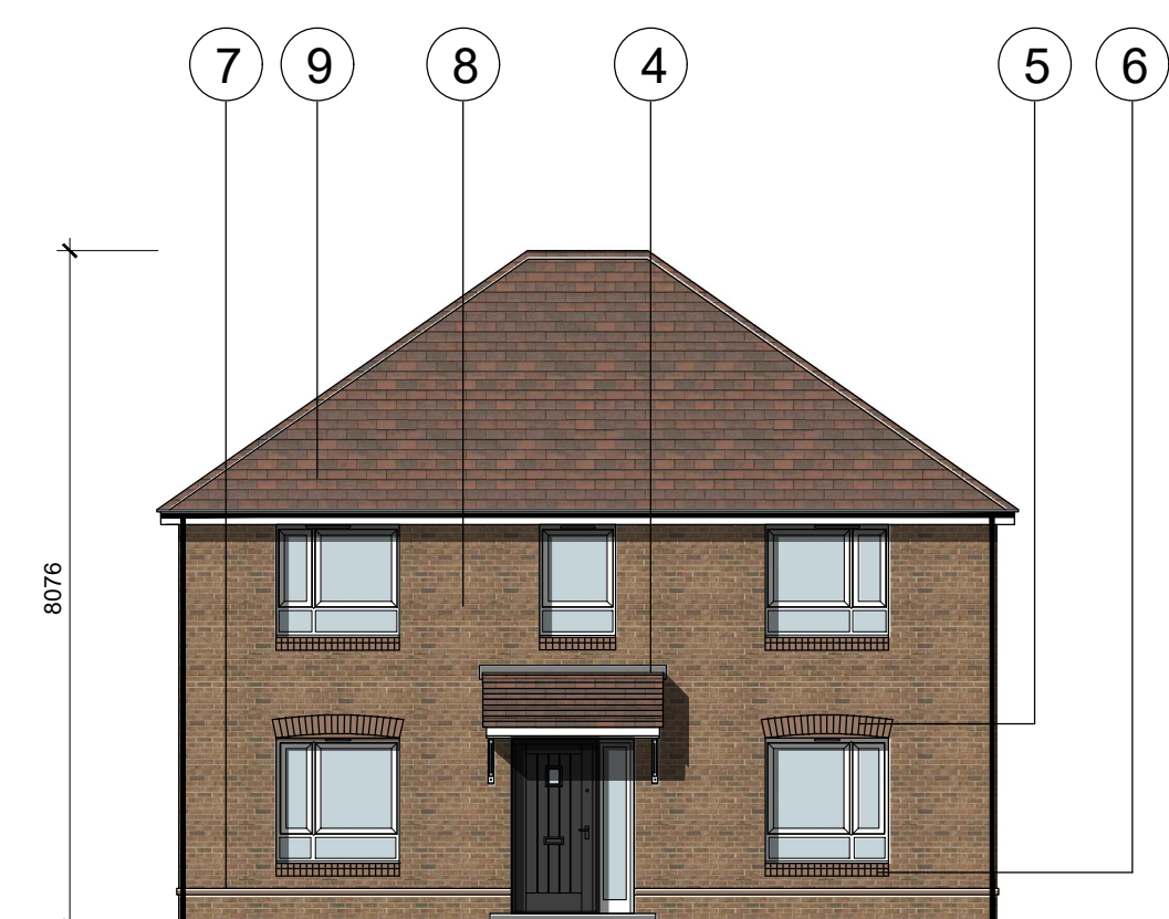
Front Elevation
