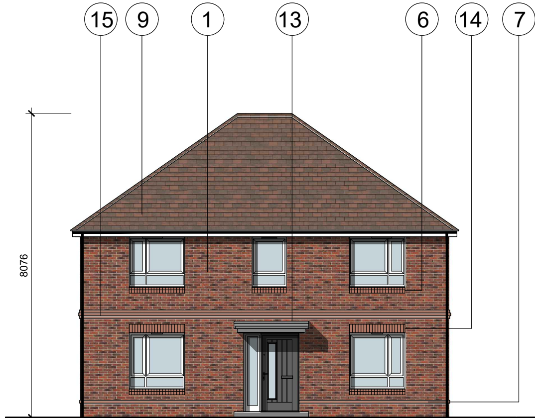
Front Elevation
