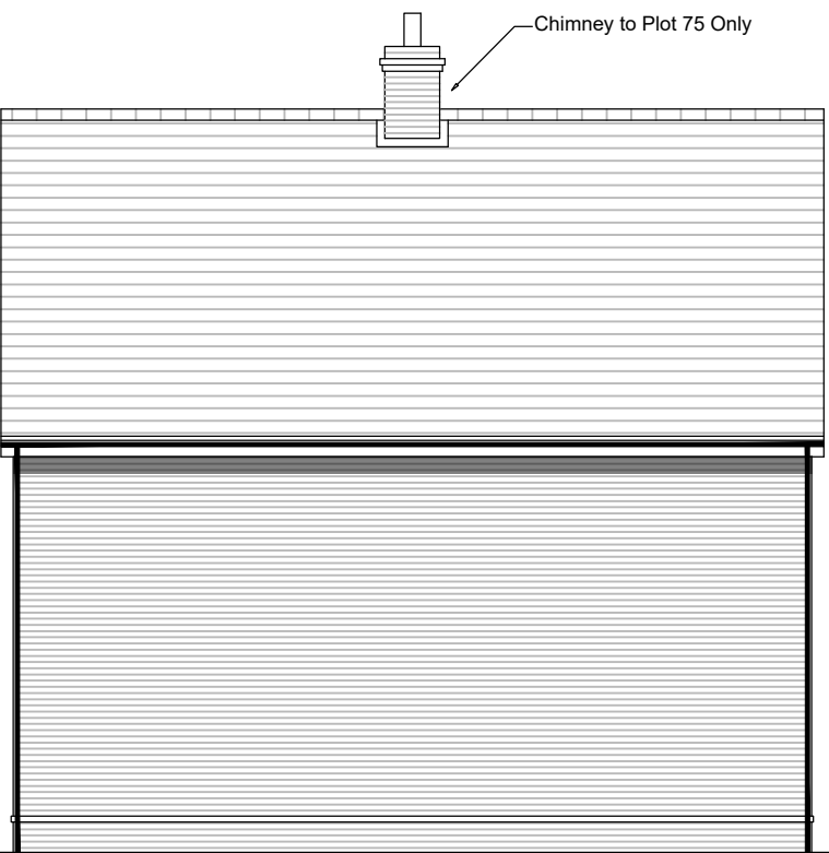
Side Elevation
