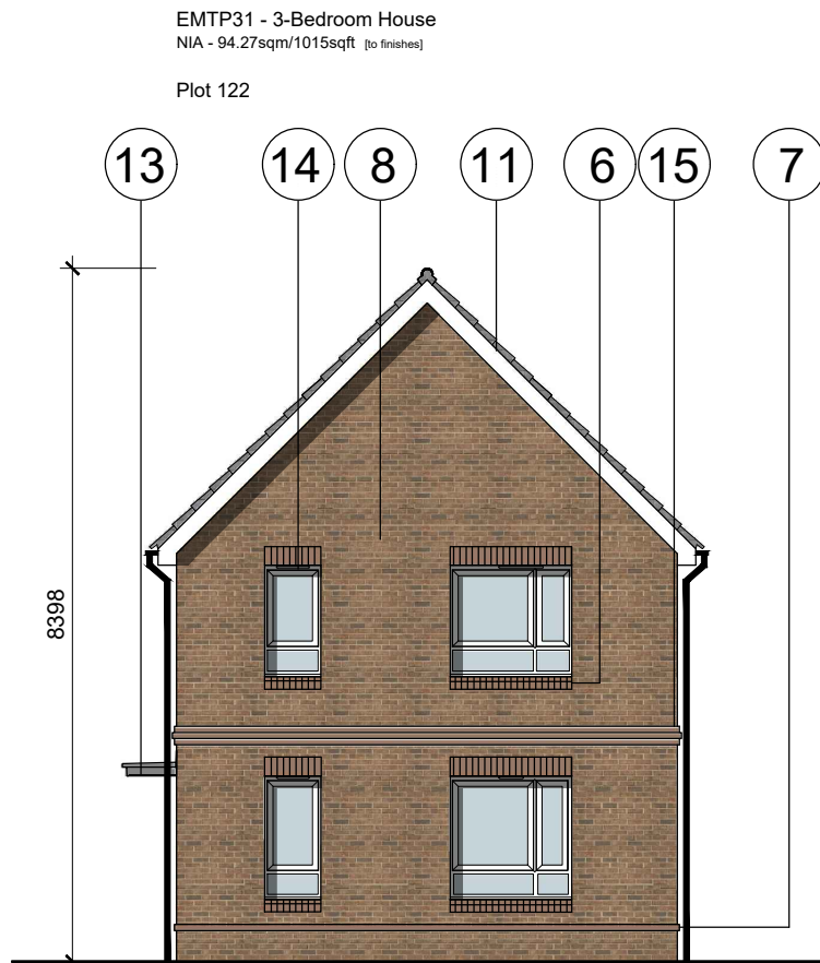
Front Elevation
