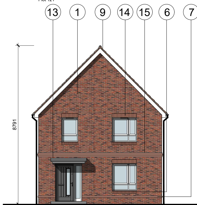
Front Elevation
