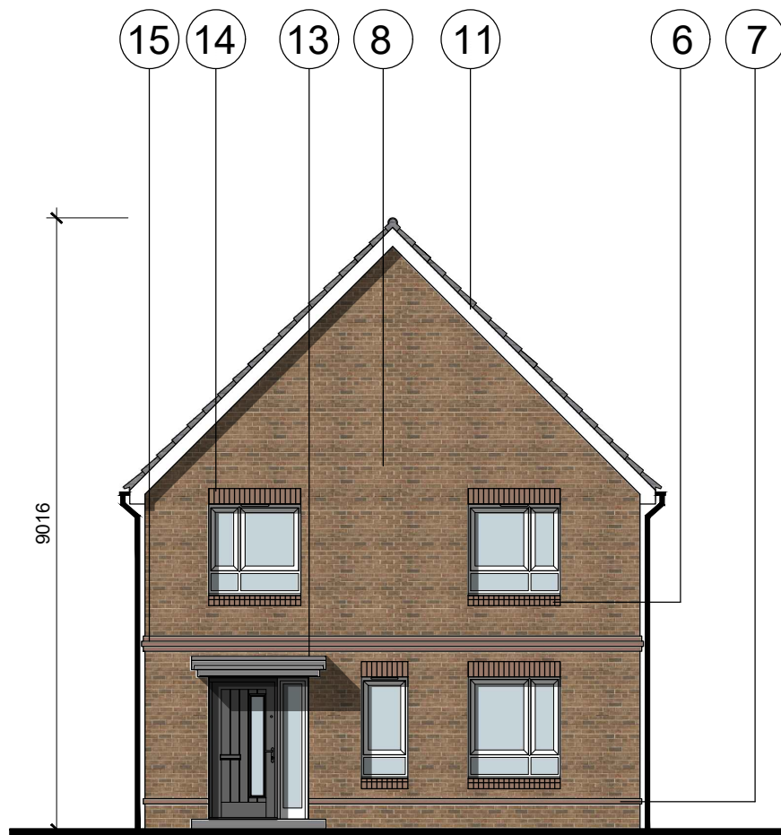
Front Elevation
