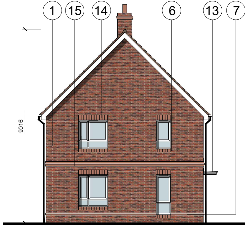
Side Elevation
