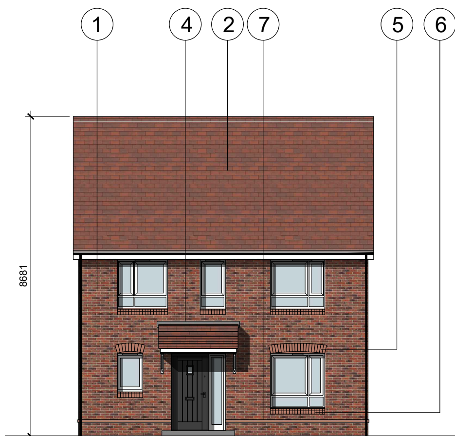
Front Elevation
