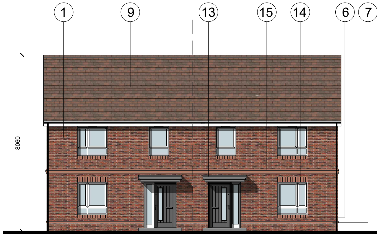
Front Elevation
