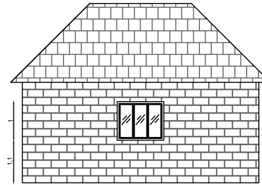
PROPOSED LEFT SIDE ELEVATION Scale 1: 100
