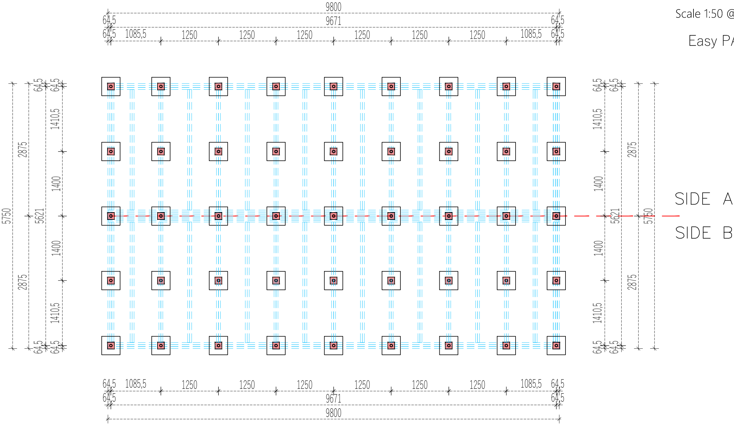
Foundation Pad Layout
