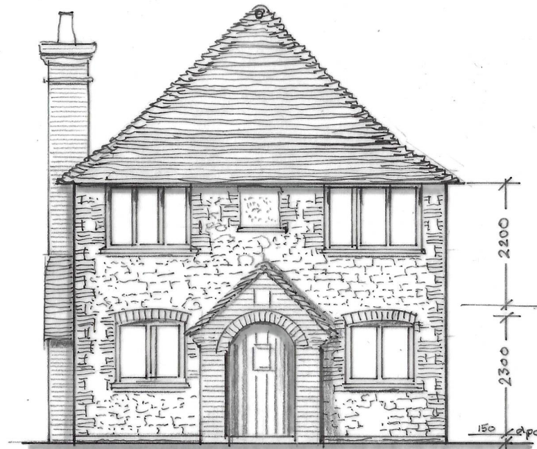
WEST ELEVATION
