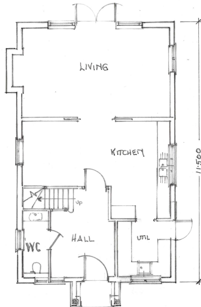
GROUND FLOOR 1:100
