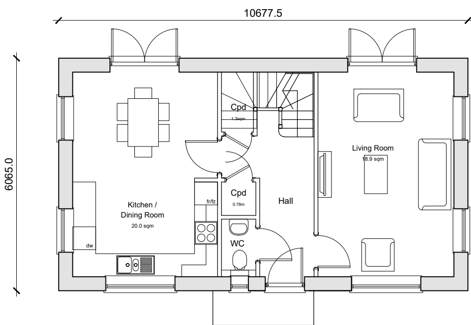
Ground Floor Plan HT08 4-Bedroom 6-Person House 106.5sqm / 1140sqft GIA (p. to be used) A minimum of 3.0 sqm storage provided in accordance with NDIS requirements.
