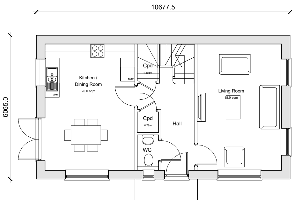
Ground Floor Plan HT07 4-Bedroom 6-Person House 106 sqm / 1140sqft GIA (p. to be used) A minimum of 3.0 sqm storage provided in accordance with NDIS requirements.
