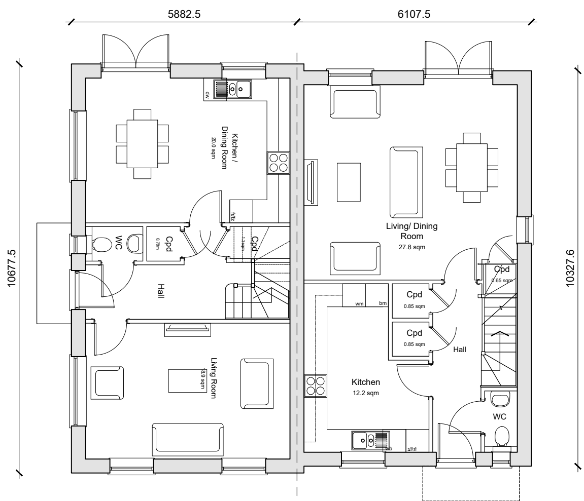
Ground Floor Plan HT07 4-Bedroom 6-Person House 106.0sqm / 1140sqft GIA (to include) A minimum of 3.0 sqm storage provided in accordance with NDIS requirements.
