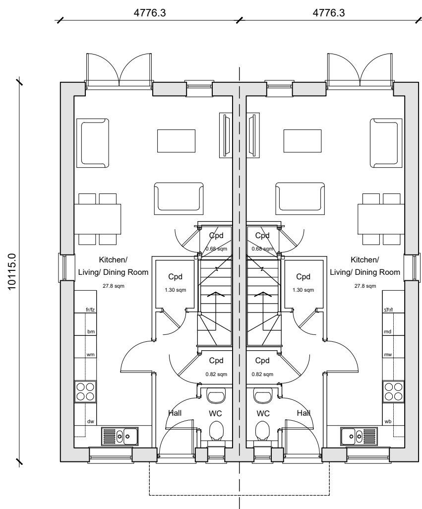
Ground Floor Plan HT01 2-Bedroom 4-Person House 79.36sqm / 854sqft GFA (to be used) A minimum of 2 sqm storage provided in accordance with NC55 requirements. Plots 26, 27
