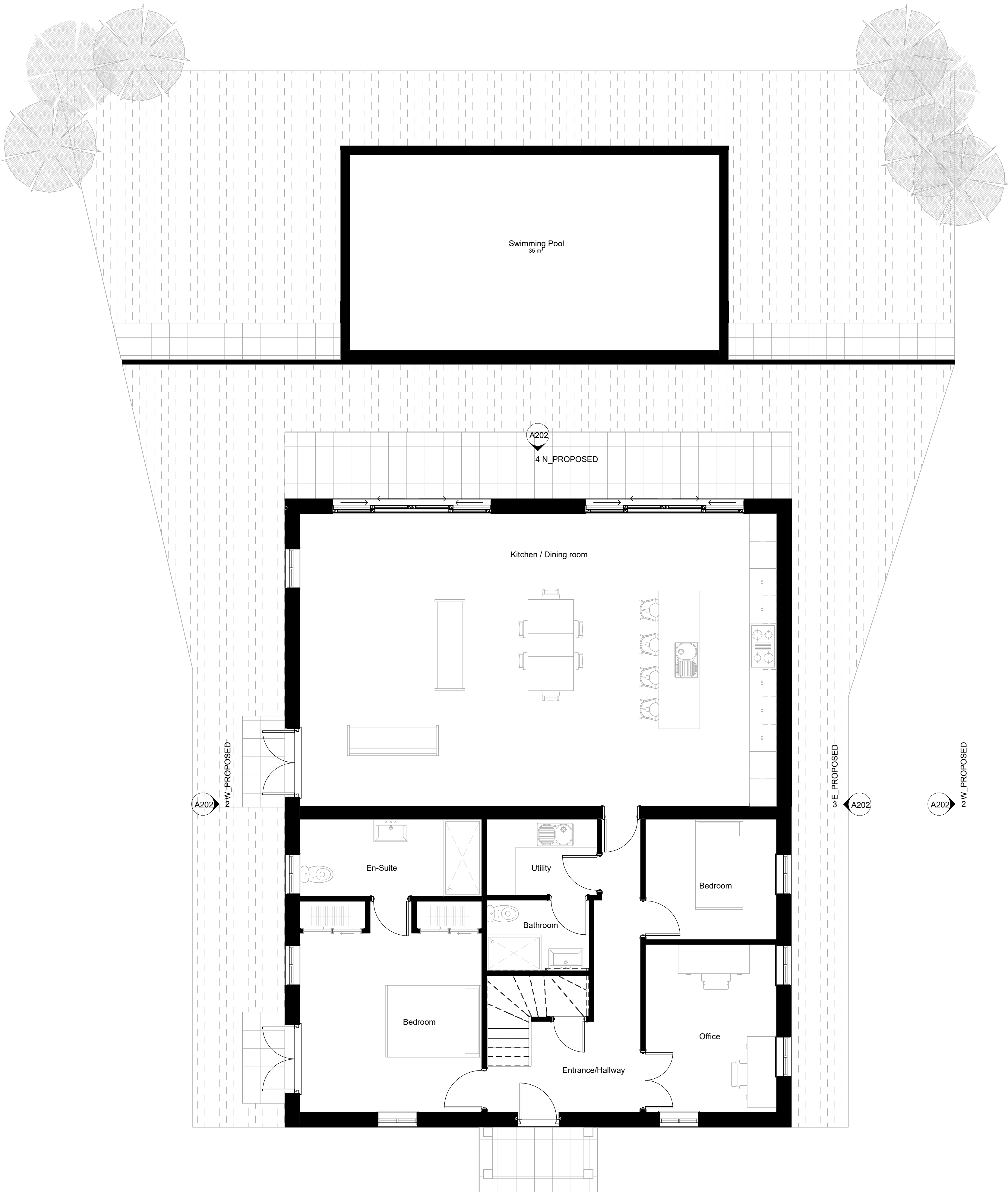
1 G_PROPOSED 1 : 50
